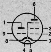
Noval B9A
